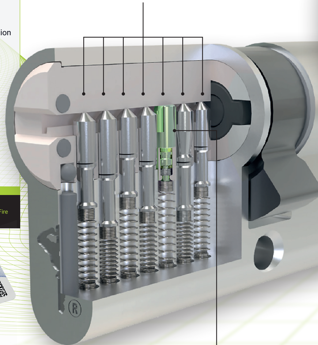
MTL™300 Telescopic Pin
